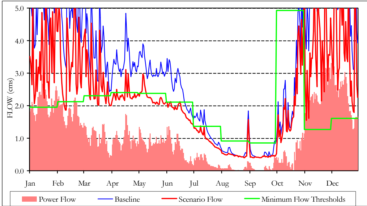
Figure 6. Hydrograph of 'Falls Creek' showing daily flows averaged over the period of record for a project scenario that meets the Guidelines. The blue solid line shows the baseline flow, the solid red line the post-project scenario (flows calculated based on flow thresholds in Hatfield et al. 2003). Pink columns indicate flows diverted down the penstock (powerflows) and the solid green line shows the monthly flow thresholds.
