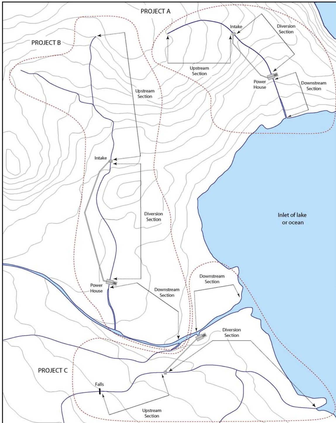
Figure 2. Examples of upstream, diversion, and downstream sections for three hypothetical hydroelectric projects.
